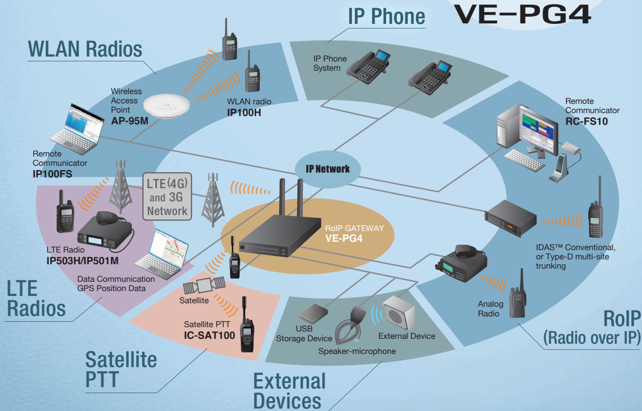
RoIP GATEWAY
